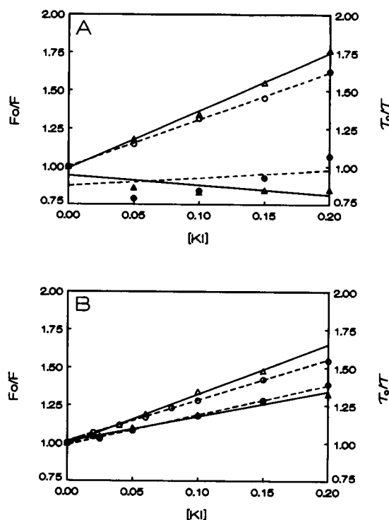
FIGURE 2 F_0/F vs. [KI] , (in molar), for NMIGG ( \triangle ) and 4-4-20 ( \blacktriangle ) and \langle\tau_0\rangle/\langle\tau\rangle vs. [KI] , (in molar), for NMIGG ( \circ ) and 4-4-20 ( \bullet ). Samples are labeled 1x with (A) FITC I and (B) FITC II.
